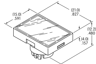
AT3006 Rectangular
