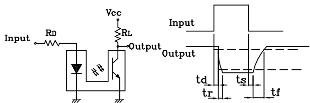
Test Circuit for Response Time
