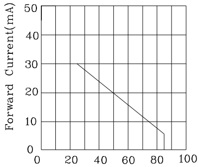
Ambient Temperature T_a ( ^{\circ} C) FORWARD CURRENT DERATING CURVE
