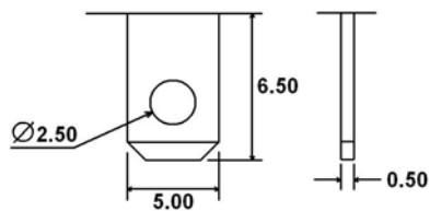
Solder Tabs
