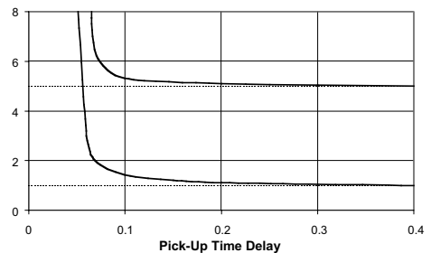
Typical Curves (WC3 Series)
