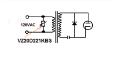
MOV In Microwave Oven
