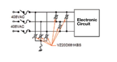
MOV for 3 Phase AC Line Protection
