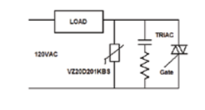
MOV in Triac Protection
