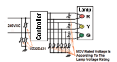
MOV In Traffic Light Protection
