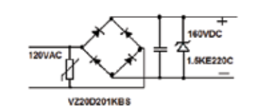
MOV in Bridge Rectifier Protection
