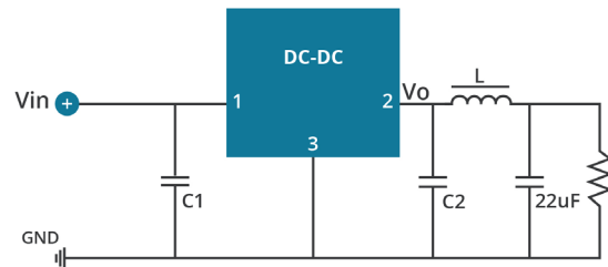
Negative Output Ripple Reduction Circuit
