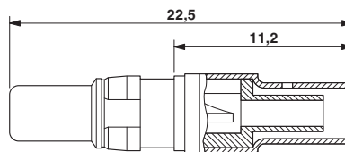
Dimensional drawing
