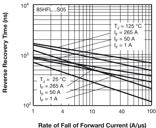
Rate of Fall of Forward Current (A/μs) Fig. 33 - Typical Reverse Recovery Time vs. Rate of Fall of Forward Current, 85HFL...S05 Series
