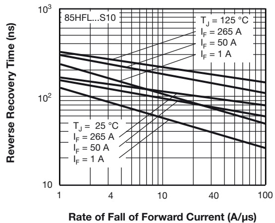
Rate of Fall of Forward Current (A/μs) Fig. 35 - Typical Reverse Recovery Time vs. Rate of Fall of Forward Current, 85HFL...S10 Series
