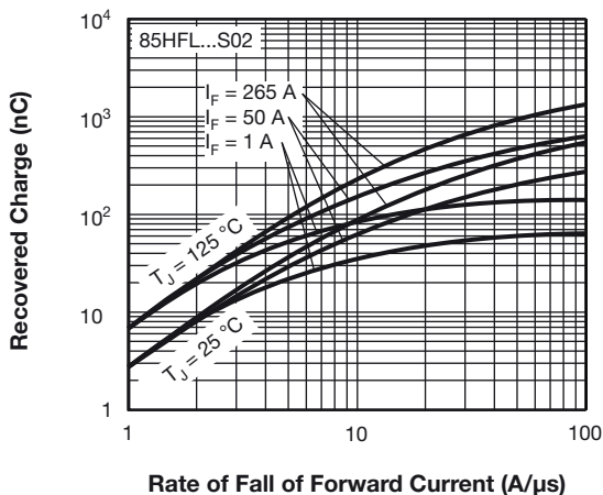
Rate of Fall of Forward Current (A/μs) Fig. 32 - Typical Recovered Charge vs. Rate of Fall of Forward Current, 85HFL...S02 Series
