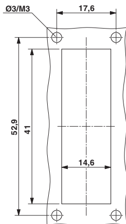
Dimensional drawing
