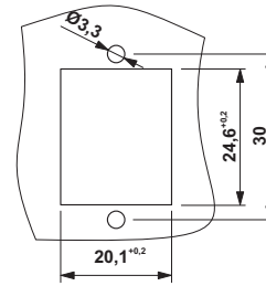
Dimensional drawing
