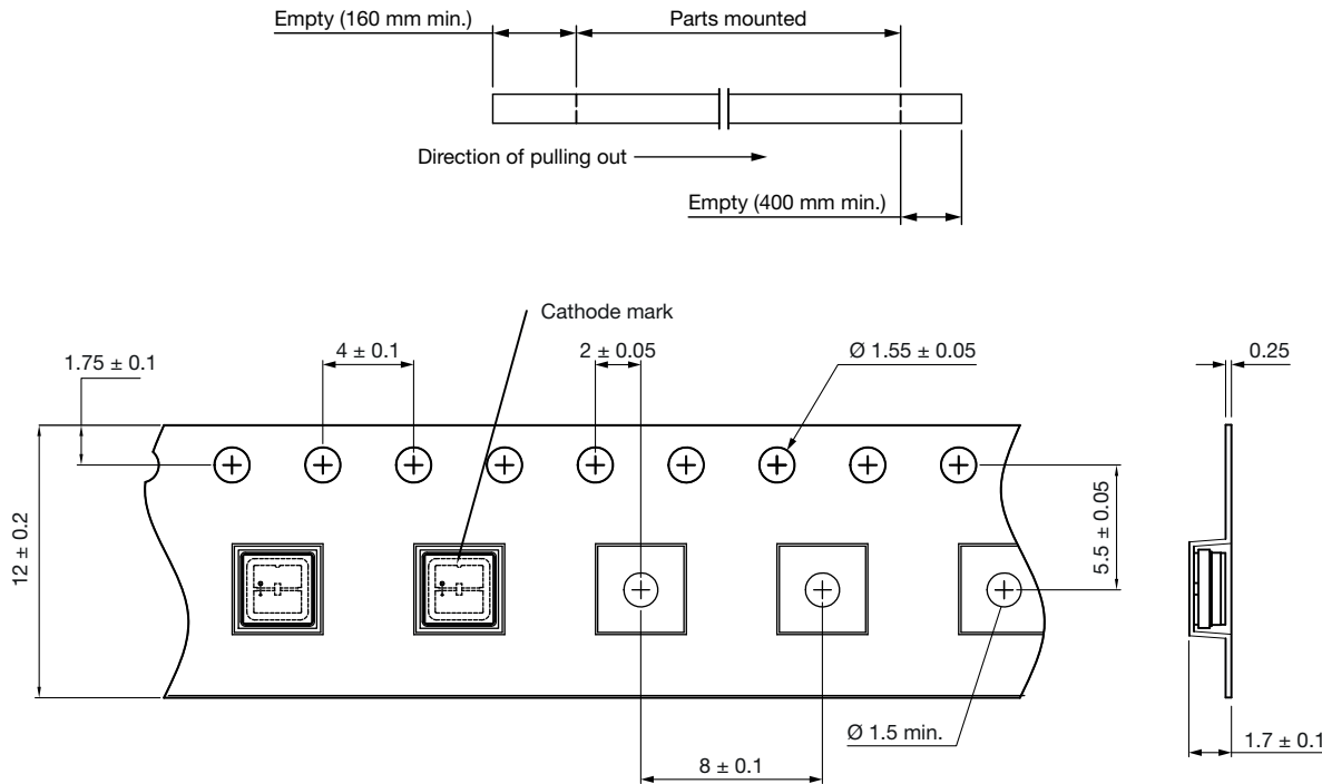
Leader and trailer tape
