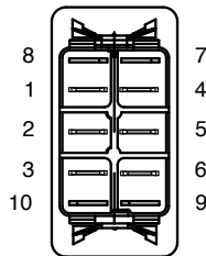
BOTTOM VIEW TERMINAL ARRANGEMENT 10 TERMINAL BASE
