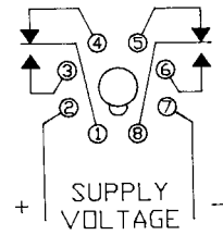
(DC POLARITY SHOWN) RB-08 or PF083A
