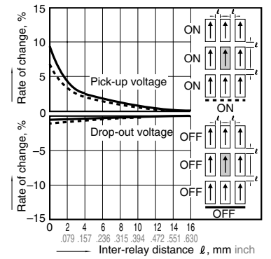
14-(3). Influence of adjacent mounting Tested sample: TXS2-4.5V, 6 pcs.
