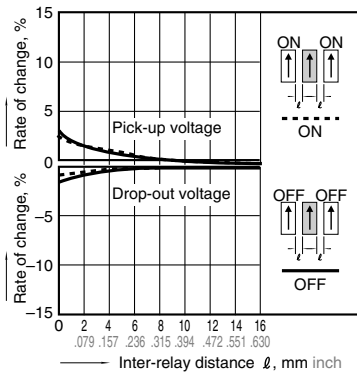
14-(1). Influence of adjacent mounting Tested sample: TXS2-4.5V, 6 pcs.
