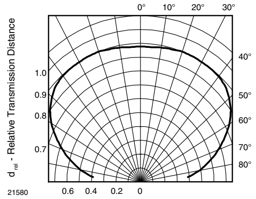
Fig. 12 - Vertical Directivity
