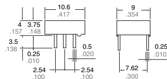
Standard PC board terminal
