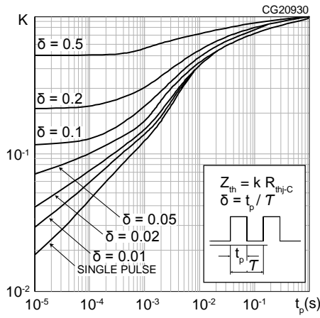
Figure 27: Thermal impedance for diode
