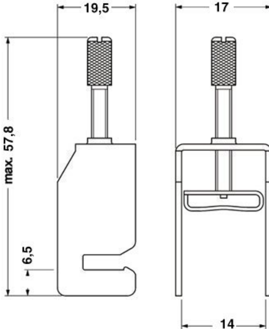
Dimensional drawing
