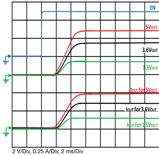
Figure 27 - Typical Turn-on Delay, Rise Time C_{OUT} = 200 \mu\text{F} , C_{IN} = 4.7 \mu\text{F} , R_{OUT} = 10 \Omega
