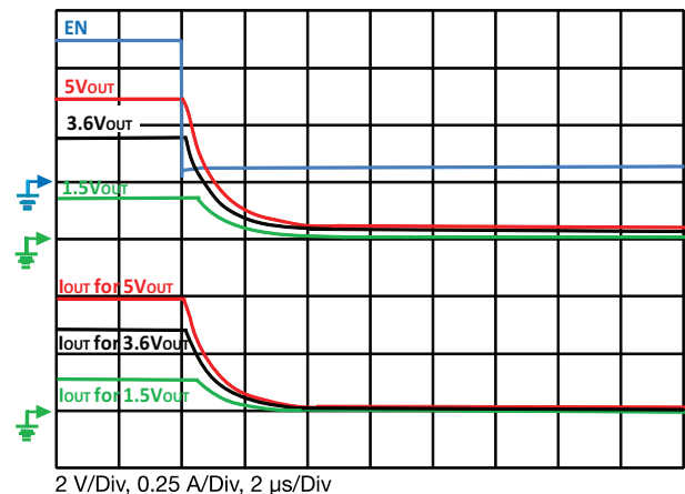
Fig. 22 - Typical Fall Time C_{OUT} = 0.1 \mu F, C_{IN} = 4.7 \mu F, R_{OUT} = 10 \Omega
