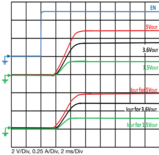
Figure 24 - Typical Turn-on Delay, Rise Time C_{OUT} = 200 \mu F , C_{IN} = 4.7 \mu F , R_{OUT} = 10 \Omega
