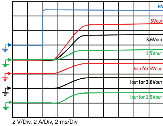
Figure 18 - Typical Turn-on Delay, Rise Time C_{OUT} = 0.1 \mu\text{F} , C_{IN} = 4.7 \mu\text{F} , I_{OUT} = 1.5 \text{ A}
