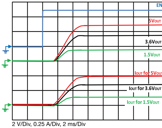
Figure 19 - Typical Turn-on Delay, Rise Time C_{OUT} = 0.1 \mu\text{F} , C_{IN} = 4.7 \mu\text{F} , R_{OUT} = 10 \Omega
