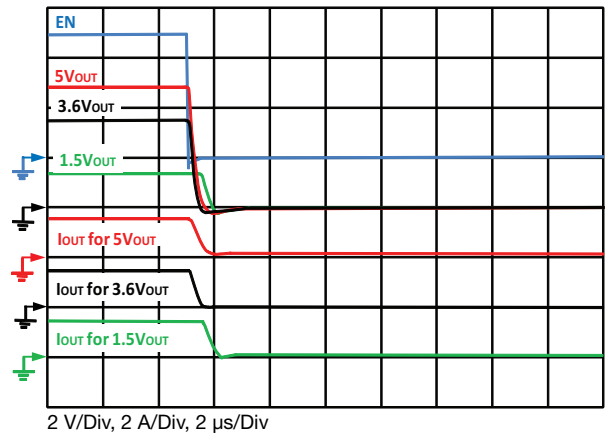
Figure 21 - Typical Fall Time C_{OUT} = 0.1 \mu\text{F} , C_{IN} = 4.7 \mu\text{F} , I_{OUT} = 1.5 \text{ A}
