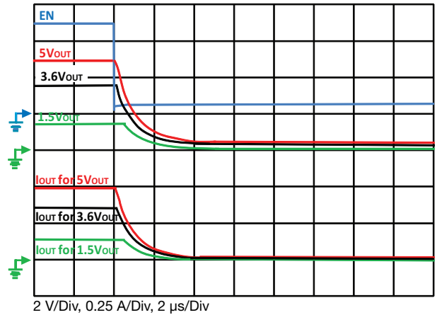
Figure 22 - Typical Fall Time C_{OUT} = 0.1 \mu\text{F} , C_{IN} = 4.7 \mu\text{F} , R_{OUT} = 10 \Omega
