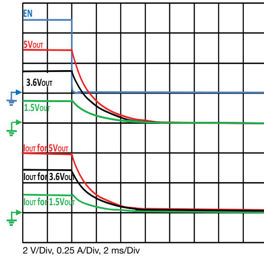
Figure 25 - Typical Fall Time C_{OUT} = 200 \mu F , C_{IN} = 4.7 \mu F , R_{OUT} = 10 \Omega
