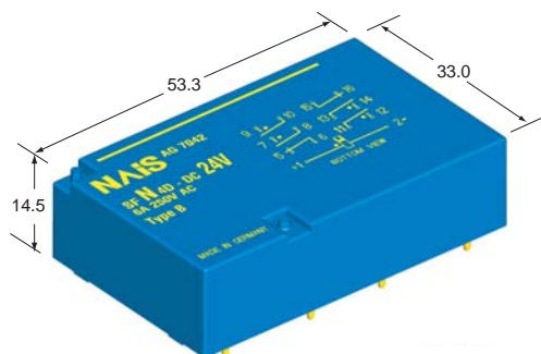
Tolerance \pm 0.3 mm Weight approx. 42 g
