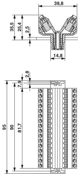
Dimensional drawing
