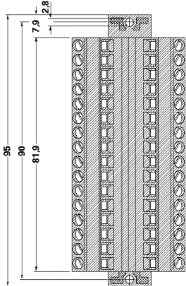
Dimensional drawing
