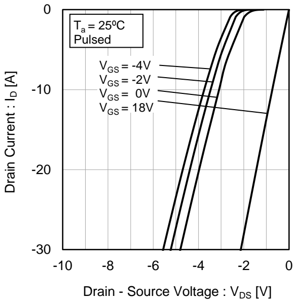
Fig.6 T_j = 25^\circ C 3rd Quadrant Characteristics
