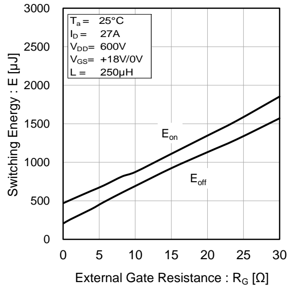
Fig.22 Typical Switching Loss vs. External Gate Resistance
