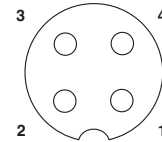
Pin assignment M12 socket, A-coded
