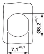
Housing cutout for M8 flush-type connector, connector, one-section
