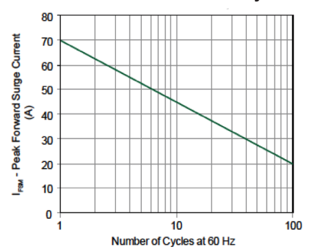
FIG.4 – Max. Non-Repetitive Forward Surge Current Uni-Directional Only
