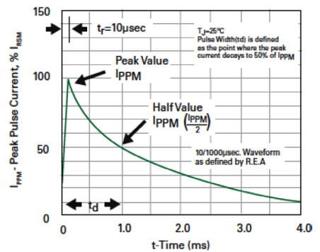
FIG.3 – Pulse Waveform
