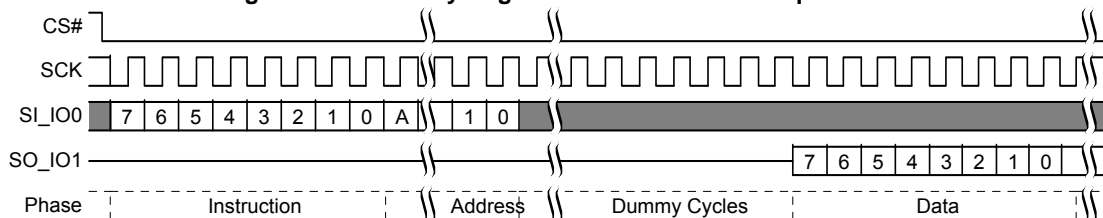
Figure 59. Read Any Register Read Command Sequence
