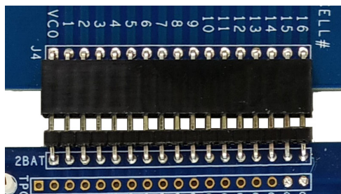
Figure 10. Cell Connection
