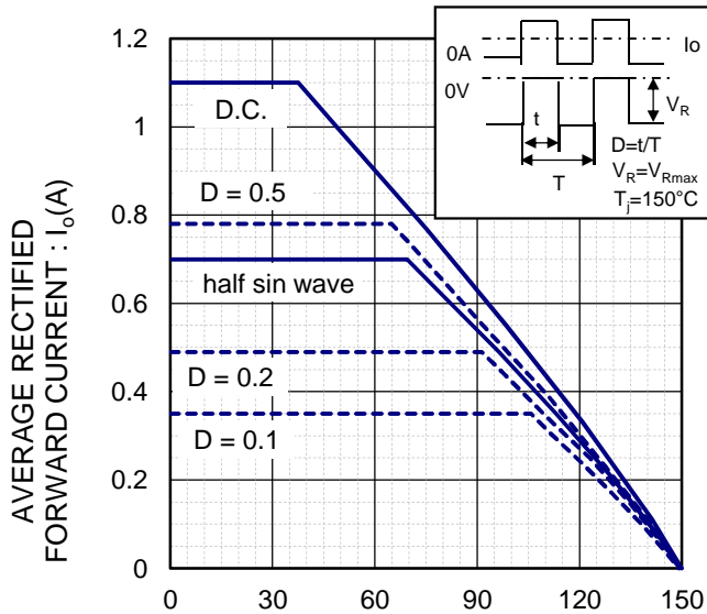
AMBIENT TEMPERATURE : T_a ( ^{\circ} C) DERATING CURVE ( I_o - T_a )
