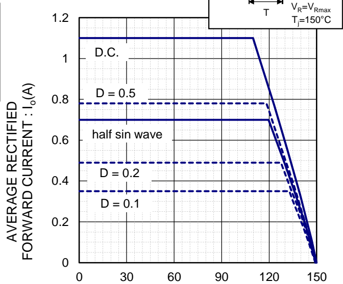
LEAD TEMPERATURE : T_l ( ^{\circ} C) DERATING CURVE ( I_o - T_l )
