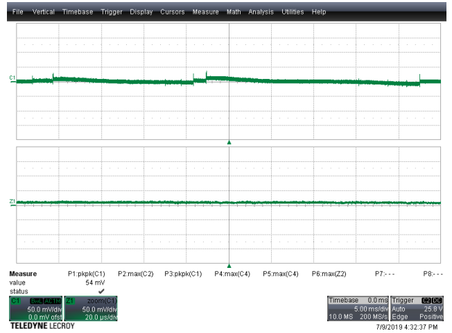
Figure 76 – Output Voltage Ripple. V_{IN} = 400 VDC, I_{OUT} = 2.5 A. Top Half: V_{OUT} , 50 mV, 5 ms / div. Bottom Half: Zoom @ 20 \mu s / div. V_{RIPPLE} = 54 mV P-P
