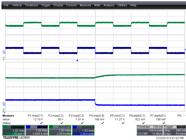
Figure 98 – Output Load Transient, 100% to 0% Load. V_{IN} = 30 \text{ VDC} , I_{OUT} = 0.85 \text{ A} to 0 A. V_{OUT(MAX)} = 12.10 \text{ V} , V_{OUT(MIN)} = 11.27 \text{ V} . Upper: V_{OUT} , 1 V, 100 ms / div. Lower: I_{OUT} , 1 A, 100 ms / div. Bottom Half: Zoom @ 2 ms / div.
