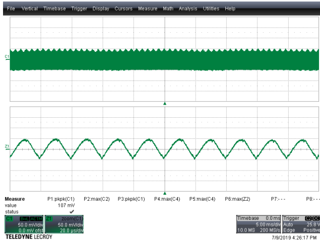
Figure 55 – Output Voltage Ripple. V_{IN} = 130 \text{ VDC} , I_{OUT} = 2.5 \text{ A} . Top Half: V_{OUT} , 50 mV, 5 ms / div. Bottom Half: Zoom @ 20 \mu\text{s} / div. V_{RIPPLE} = 107 \text{ mV}_{p-p}
