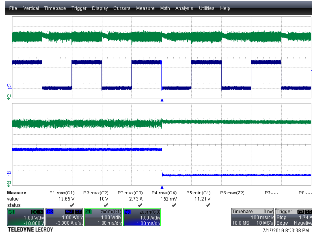
Figure 101 – Output Load Transient, 100% to 0% Load. V_{IN} = 400 \text{ VDC} , I_{OUT} = 2.5 \text{ A} to 0 A. V_{OUT(MAX)} = 12.65 \text{ V} , V_{OUT(MIN)} = 11.21 \text{ V} . Upper: V_{OUT} , 1 V, 100 ms / div. Lower: I_{OUT} , 1 A, 100 ms / div. Bottom Half: Zoom @ 1 ms / div.
