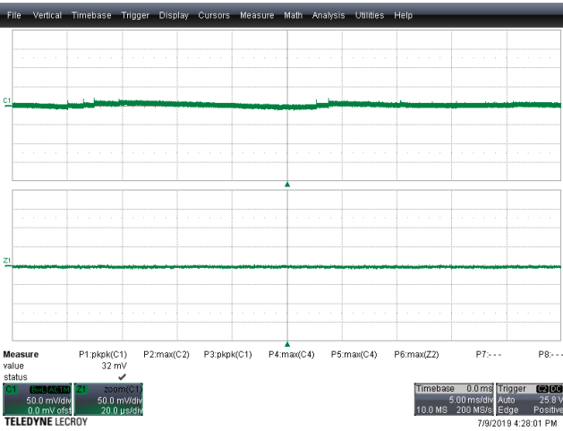
Figure 75 – Output Voltage Ripple. V_{IN} = 130 VDC, I_{OUT} = 2.5 A. Top Half: V_{OUT} , 50 mV, 5 ms / div. Bottom Half: Zoom @ 20 \mu s / div. V_{RIPPLE} = 32 mV P-P
