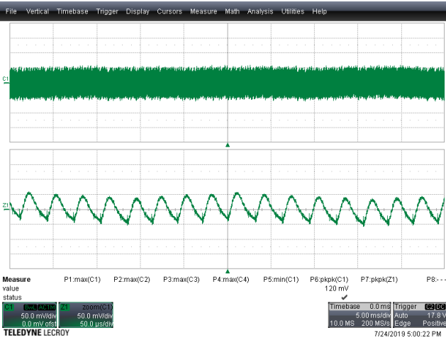
Figure 84 – Output Voltage Ripple. V_{IN} = 130 \text{ VDC} , I_{OUT} = 1.25 \text{ A} . Top Half: V_{OUT} , 50 mV, 5 ms / div. Bottom Half: Zoom @ 50 \mu\text{s} / div. V_{RIPPLE} = 120 \text{ mV}_{p-p}
