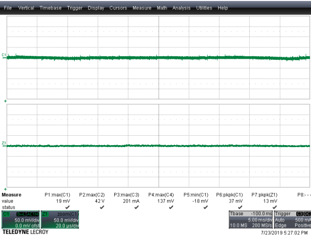
Figure 73 – Output Voltage Ripple. V_{IN} = 30 VDC, I_{OUT} = 0.85 A. Top Half: V_{OUT} , 50 mV, 5 ms / div. Bottom Half: Zoom @ 20 \mu s / div. V_{RIPPLE} = 37 mV P-P
