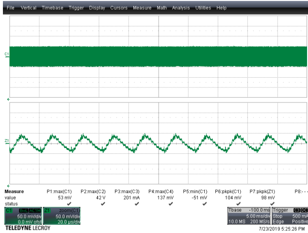
Figure 53 – Output Voltage Ripple. V_{IN} = 30 \text{ VDC} , I_{OUT} = 0.85 \text{ A} . Top Half: V_{OUT} , 50 mV, 5 ms / div. Bottom Half: Zoom @ 20 \mu\text{s} / div. V_{RIPPLE} = 104 \text{ mV}_{p-p}
