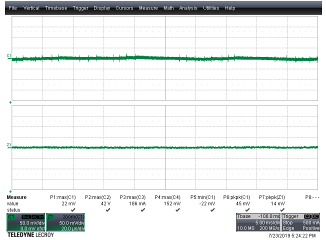
Figure 74 – Output Voltage Ripple. V_{IN} = 60 VDC, I_{OUT} = 1.25 A. Top Half: V_{OUT} , 50 mV, 5 ms / div. Bottom Half: Zoom @ 20 \mu s / div. V_{RIPPLE} = 45 mV P-P
