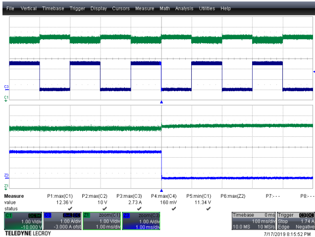
Figure 100 – Output Load Transient, 100% to 0% Load. V_{IN} = 130 \text{ VDC} , I_{OUT} = 2.5 \text{ A} to 0 A. V_{OUT(MAX)} = 12.36 \text{ V} , V_{OUT(MIN)} = 11.34 \text{ V} . Upper: V_{OUT} , 1 V, 100 ms / div. Lower: I_{OUT} , 1 A, 100 ms / div. Bottom Half: Zoom @ 1 ms / div.
