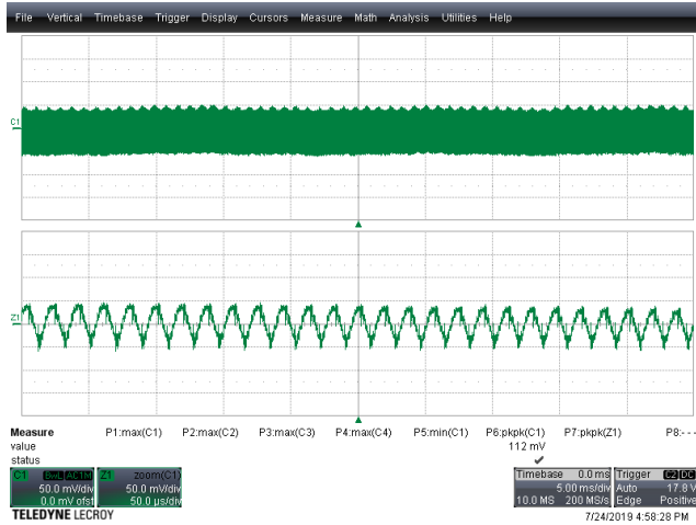
Figure 78 – Output Voltage Ripple. V_{IN} = 130 \text{ VDC} , I_{OUT} = 2.5 \text{ A} . Top Half: V_{OUT} , 50 mV, 5 ms / div. Bottom Half: Zoom @ 50 μs / div. V_{RIPPLE} = 112 \text{ mV}_{P-P}
