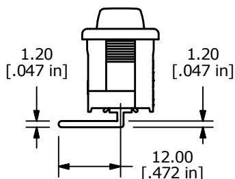
"R" TERMINAL
