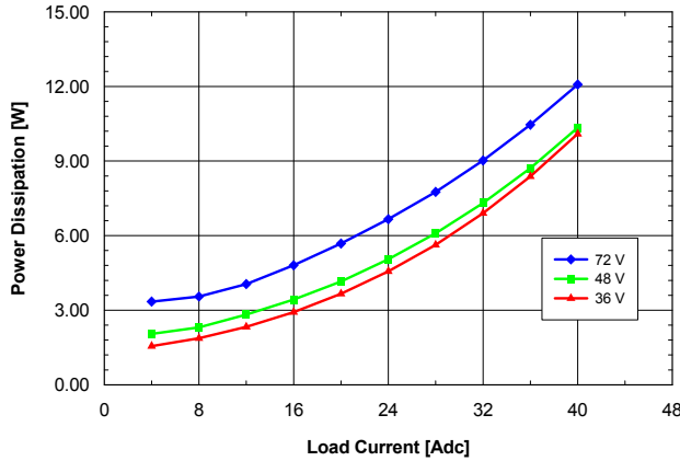
Fig. 1.2V.5: Power dissipation vs. load current and input voltage for QME48T40012 converter mounted horizontally with air flowing from pin 1 to pin 3 at a rate of 300 LFM (1.5 m/s) and T_a = 25\text{ }^\circ\text{C} .
