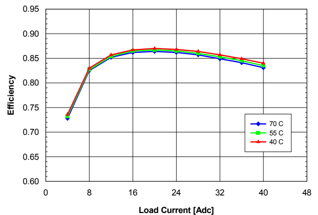
Fig. 1.5V.4: Efficiency vs. load current and ambient temperature for QME48T40015 converter mounted horizontally with V_{in} = 48 V and air flowing from pin 1 to pin 3 at a rate of 200 LFM (1.0 m/s).
