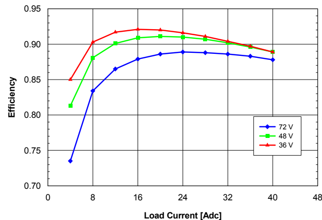
Fig. 2.5V.3: Efficiency vs. load current and input voltage for QME48T40025 converter mounted horizontally with air flowing from pin 1 to pin 3 at a rate of 300 LFM (1.5 m/s) and T_a = 25 °C.
