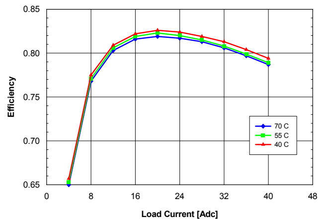
Fig. 1.0V.4: Efficiency vs. load current and ambient temperature for QME48T40010 converter mounted horizontally with V_{in} = 48 V and air flowing from pin 1 to pin 3 at a rate of 200 LFM (1.0 m/s).
