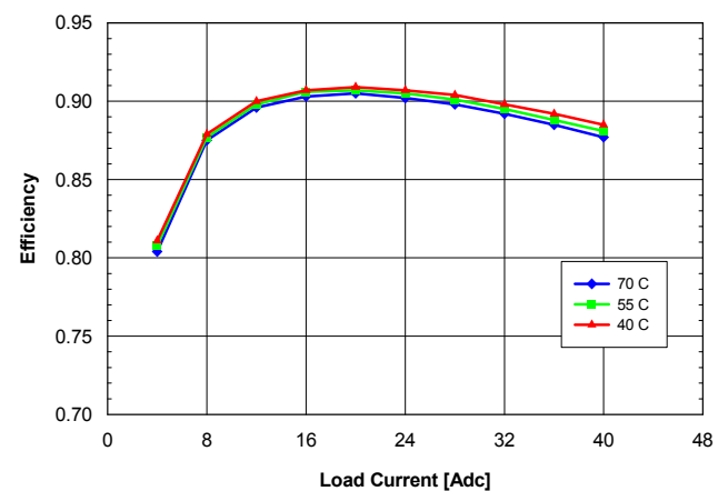
Fig. 2.5V.4: Efficiency vs. load current and ambient temperature for QME48T40025 converter mounted horizontally with V_{in} = 48 V and air flowing from pin 1 to pin 3 at a rate of 200 LFM (1.0 m/s).
