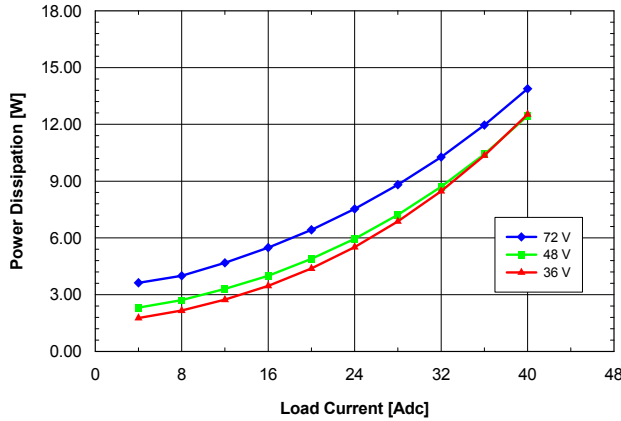
Fig. 2.5V.5: Power dissipation vs. load current and input voltage for QME48T40025 converter mounted horizontally with air flowing from pin 1 to pin 3 at a rate of 300 LFM (1.5 m/s) and T_a = 25\text{ }^\circ\text{C} .
