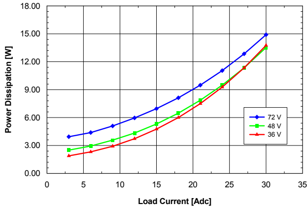
Fig. 3.3V.5: Power dissipation vs. load current and input voltage for QME48T40033 converter mounted horizontally with air flowing from pin 1 to pin 3 at a rate of 300 LFM (1.5 m/s) and T_a = 25\text{ }^\circ\text{C} .
