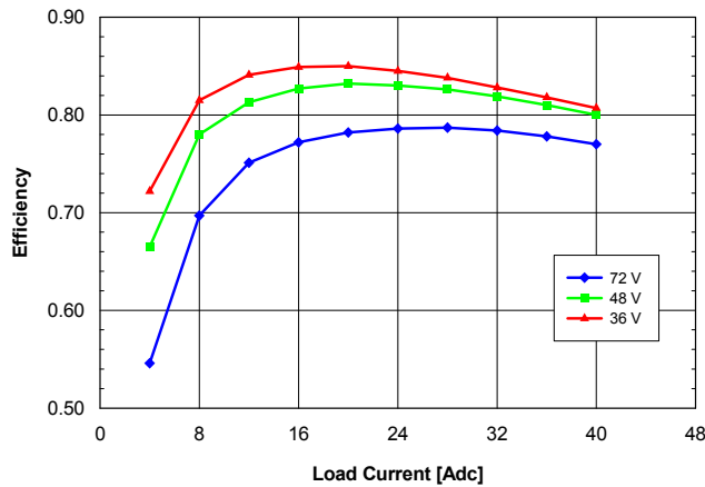
Fig. 1.0V.3: Efficiency vs. load current and input voltage for QME48T40010 converter mounted horizontally with air flowing from pin 1 to pin 3 at a rate of 300 LFM (1.5 m/s) and T_a = 25 °C.
