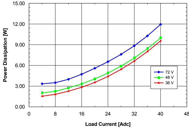
Fig. 1.0V.5: Power dissipation vs. load current and input voltage for QME48T40010 converter mounted horizontally with air flowing from pin 1 to pin 3 at a rate of 300 LFM (1.5 m/s) and T_a = 25\text{ }^\circ\text{C} .
