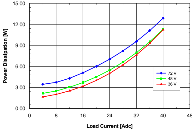
Fig. 1.8V.5: Power dissipation vs. load current and input voltage for QME48T40018 converter mounted horizontally with air flowing from pin 1 to pin 3 at a rate of 300 LFM (1.5 m/s) and T_a = 25\text{ }^\circ\text{C} .
