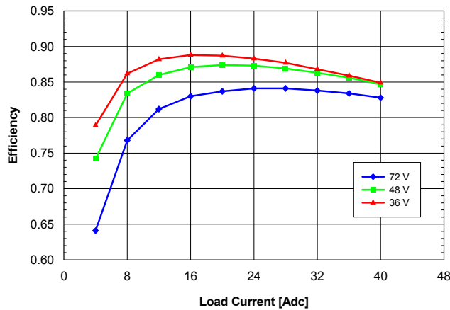
Fig. 1.5V.3: Efficiency vs. load current and input voltage for QME48T40015 converter mounted horizontally with air flowing from pin 1 to pin 3 at a rate of 300 LFM (1.5 m/s) and T_a = 25 °C.
