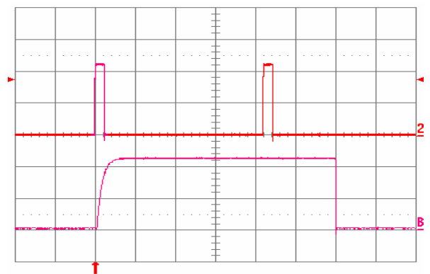
Fig. 1.8V.16: Load current (top trace, 20 A/div., 50 ms/div.) into a 10 m\Omega short circuit during restart, at V_{in} = 48 V. Bottom trace (20 A/div., 2 ms/div.) is an expansion of the on-time portion of the top trace.
