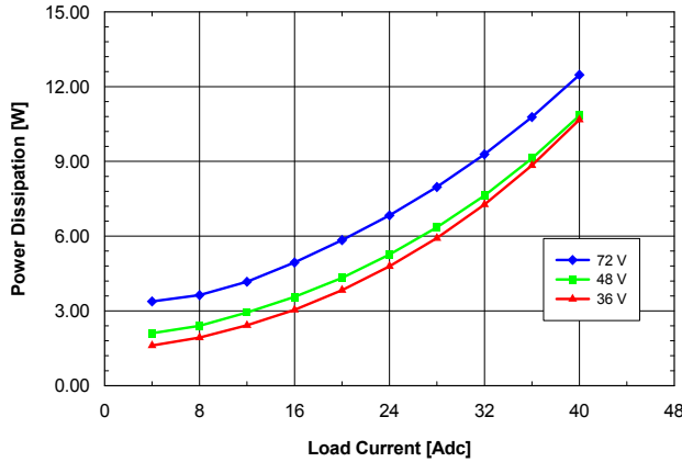
Fig. 1.5V.5: Power dissipation vs. load current and input voltage for QME48T40015 converter mounted horizontally with air flowing from pin 1 to pin 3 at a rate of 300 LFM (1.5 m/s) and T_a = 25\text{ }^\circ\text{C} .
