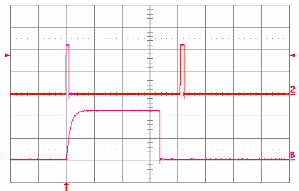
Fig. 3.3V.16: Load current (top trace, 20 A/div., 50 ms/div.) into a 10 m\Omega short circuit during restart, at V_{in} = 48 V. Bottom trace (20 A/div., 2 ms/div.) is an expansion of the on-time portion of the top trace.
