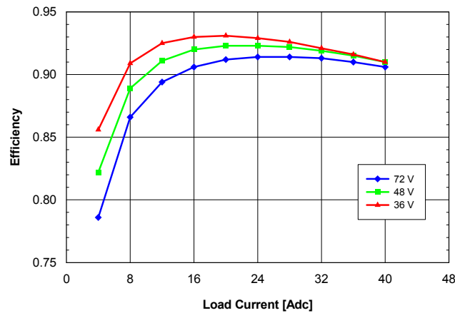
Fig. 3.3V.3: Efficiency vs. load current and input voltage for QME48T40033 converter mounted horizontally with air flowing from pin 1 to pin 3 at a rate of 300 LFM (1.5 m/s) and T_a = 25 °C.
