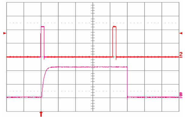
Fig. 1.5V.16: Load current (top trace, 20 A/div., 50 ms/div.) into a 10 m\Omega short circuit during restart, at V_{in} = 48 V. Bottom trace (20 A/div., 2 ms/div.) is an expansion of the on-time portion of the top trace.
