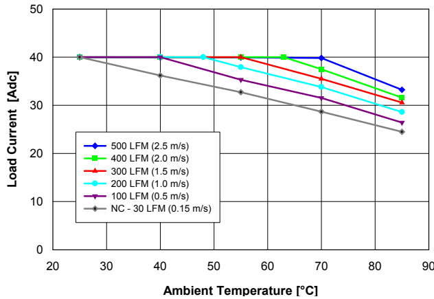
Fig. 3.3V.1: Available load current vs. ambient air temperature and airflow rates for QME48T40033 converter with G height pins mounted vertically with air flowing from pin 1 to pin 3, MOSFET temperature \leq 120 °C, V_{in} = 48 V.
