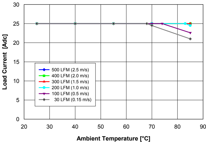
Fig. 1: Available load current vs. ambient air temperature and air-flow rates for Q48T25015 converter mounted vertically with air flowing from pin 3 to pin 1, MOSFET temperature \leq 120^{\circ}\text{C} , V_{in} = 54\text{ V} .
