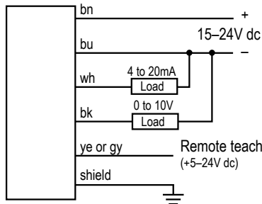
Sensor with Attached Cable
