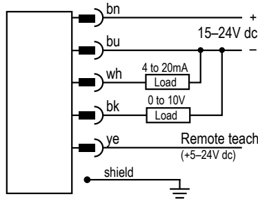
Sensor with 5-pin Mini-style QD
