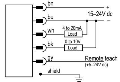
Sensor with 5-pin Euro-style QD
