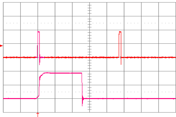
Fig. 27: Load current (top trace, 20 A/div, 20 ms/div) into a 10 mΩ short circuit during restart, at V_{in} = 24 V. Bottom trace (20 A/div, 1 ms/div) is an expansion of the on-time portion of the top trace.
