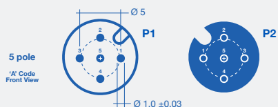
5 PINS A-CODED
