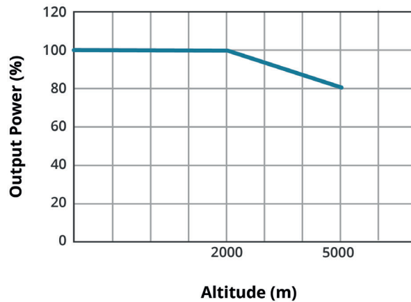
ALTITUDE DERATING CURVE (25°C)
