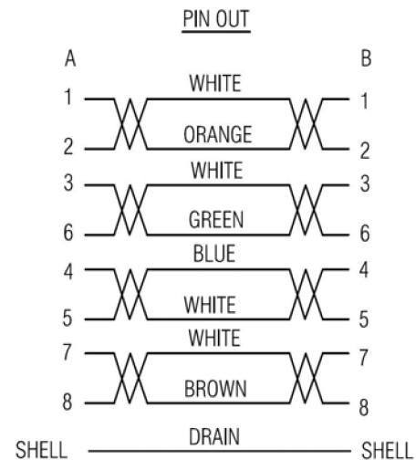
CAT 6A FLAT {32AWG(7/0.08BARE COPPER)WITH特多龙丝/150D*1P+D(7/01TIN COPPER)+A}*4C
