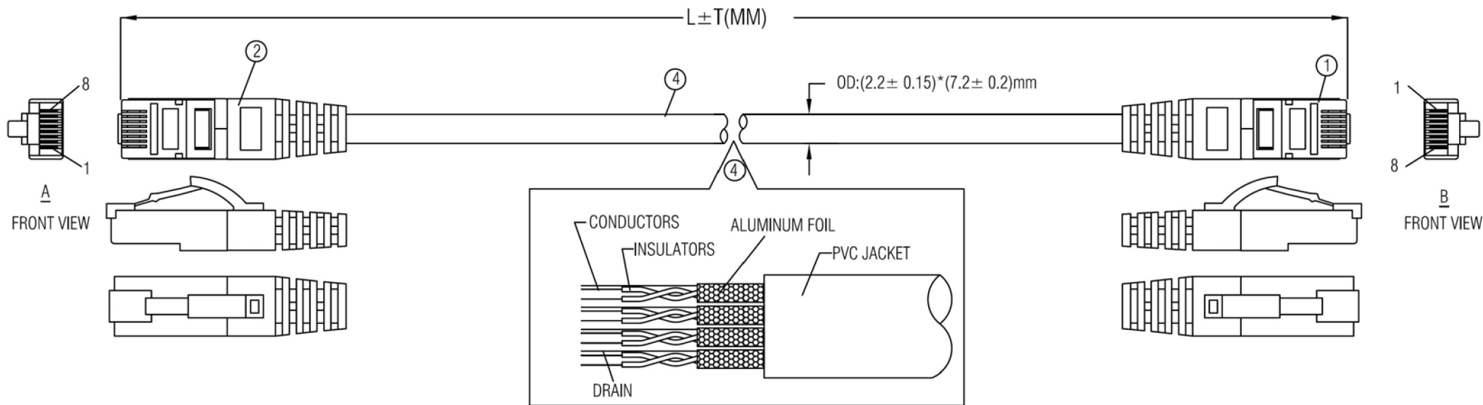
CAT 6A FLAT {32AWG(7/0.08BARE COPPER)WITH特多龙丝/150D*1P+D(7/01TIN COPPER)+A}*4C
