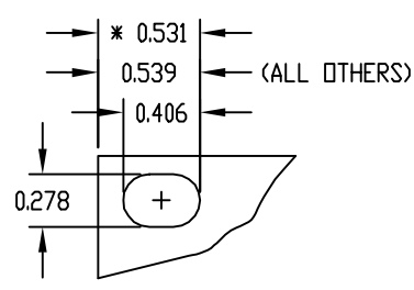
NOTCH DETAIL
