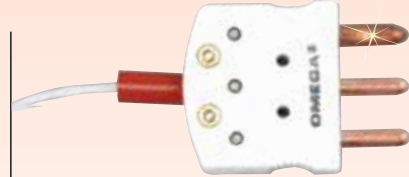
Heavy-Duty Connector OTP-U-M (e.g., RTD-2-F3102-36-G-OTP)
