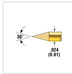
POGO-1L18-S
