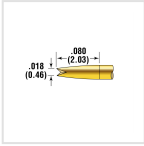
POGO-1UN
