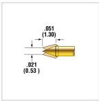
POGO-1I35-S
