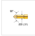
POGO-1T1
