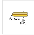
POGO-1T24
