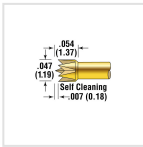
POGO-1I8-S
