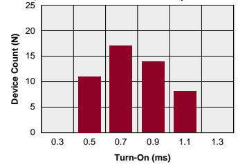
LAA127 Typical Turn-On Time (N=50 Ambient Temperature = 25°C) (Load Current = 200mADC; I F = 5mADC)
