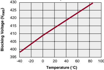
TS117 Typical Blocking Voltage vs. Temperature
