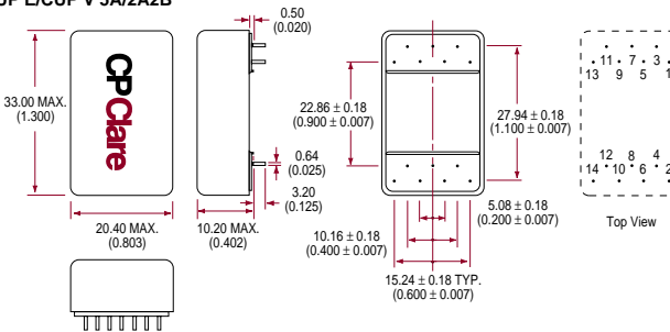
CUP E/CUP V 5A/2A2B
