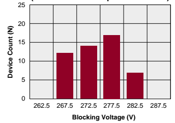
LAA127 Typical Blocking Voltage Distribution (N=50 Ambient Temperature = 25°C)
