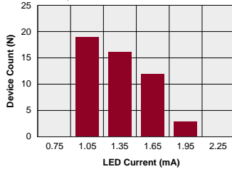
LAA127 Typical I F for Switch Dropout (N=50 Ambient Temperature = 25°C) (Load Current = 200mADC)
