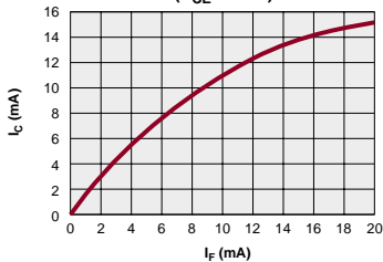
ITC117P/ITC135P/ITC137P Darlington Transistor Typical Collector Current vs. Forward Current ( V_{CE} = 0.5V )
