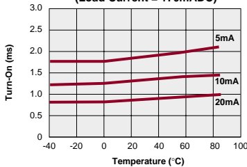
LAA125 Typical Turn-On vs. Temperature (Load Current = 170mAADC)
