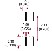
MRF8 J Lead (Lead Option -02)
