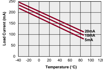
LBA120L - Form A Typical Load Current vs. Temperature
