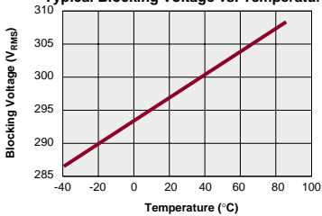
LBB126 Typical Blocking Voltage vs. Temperature
