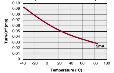
PAA110L Typical Turn-Off vs. Temperature (Load Current = 150mA)
