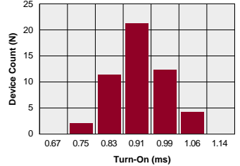
XBB170 Typical Turn-On Time (N=50 Ambient Temperature = 25°C) (Load Current = 100mADC)
