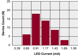
IAB110P - FormA Typical I F for Switch Dropout (N=50 Ambient Temperature = 25°C) (Load Current = 100mA DC)
