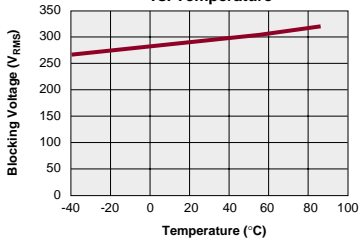
LAA127 Typical Blocking Voltage vs. Temperature
