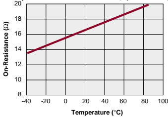
LBA110L - FormA Typical On-Resistance vs. Temperature (Load Current = 120mADC; I_F = 5\text{mADC} )
