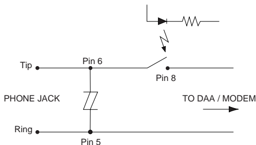
Figure 1. Typical Telecommunications Application
