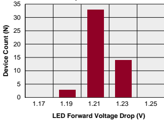
LAA127 Typical LED Forward Voltage Drop (N=50 Ambient Temperature = 25°C) I F = 5mADC
