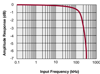
Figure 2A. Photoconductive Amplitude Response
