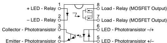
TS120 Pinout
