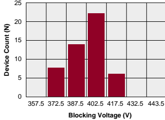
IAB110P - FormB Typical Blocking Voltage Distribution (N=50 Ambient Temperature = 25°C)
