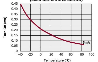
LAA127 Typical Turn-Off vs. Temperature (Load Current = 200mADC)
