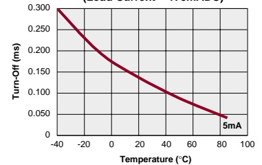
LAA125 Typical Turn-Off vs. Temperature (Load Current = 170mAADC)
