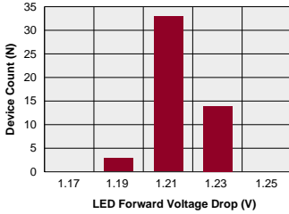
LAA125 Typical LED Forward Voltage Drop (N=50 Ambient Temperature = 25°C) I F = 5mAADC
