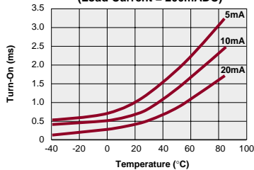
LAA127 Typical Turn-On vs. Temperature (Load Current = 200mADC)
