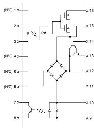
Figure 1. 16 Pin SOIC Package
