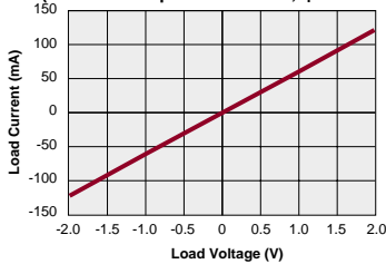
LBA110L - FormA Typical Load Current vs. Load Voltage (Ambient Temperature = 25°C; I_F = 5\text{mADC} )
