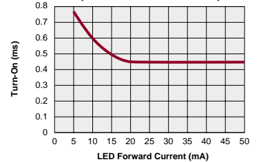
LBA127 - FormA Typical Turn-On vs. LED Forward Current (Load Current = 170mADC)
