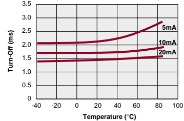
LBA127 - FormB Typical Turn-Off vs. Temperature (Load Current = 170mADC)
