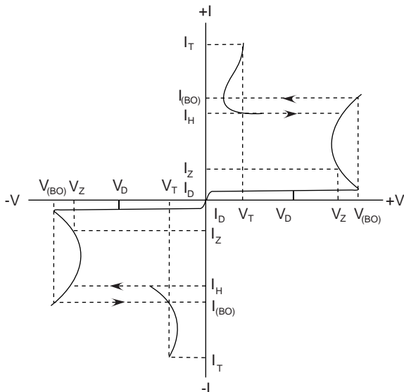
Figure 2. Transfer Characteristics of the SSSA
