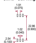
SMR6 - Gull Wing
