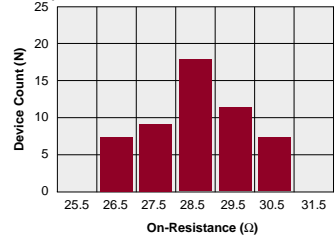
IAB110P - FormB Typical On-Resistance Distribution (N=50 Ambient Temperature = 25°C) (Load Current = 100mA DC, I F = 5mA DC)
