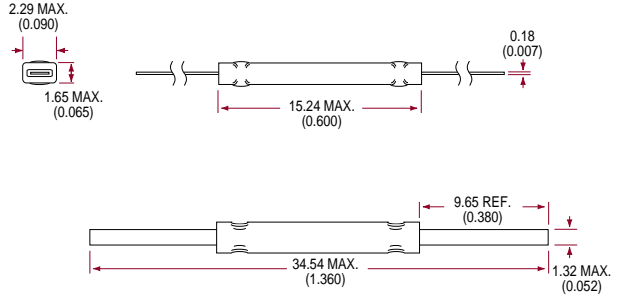
DYAD®
