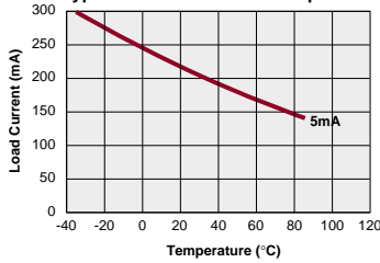
LAA127 Typical Load Current vs. Temperature
