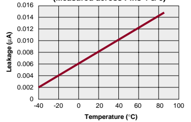
XAA170 Typical Leakage vs. Temperature (Measured across Pins 4 & 6)
