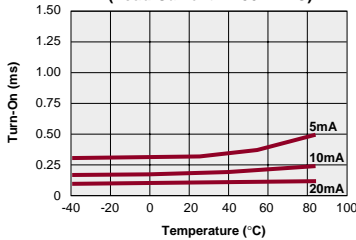
PAA110L Typical Turn-On vs. Temperature (Load Current = 150mA)
