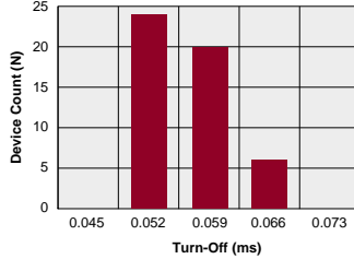
PAA110L Typical Turn-Off Time (N=50 Ambient Temperature = 25°C) (Load Current = 150mA; I F = 5mA)
