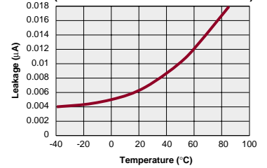
LAA127 Typical Leakage vs. Temperature (Measured across Pins 5 & 6 or 7 & 8)
