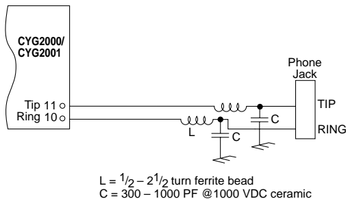
Figure 10. EMI Considerations
