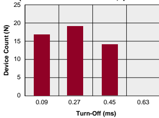
LAA127 Typical Turn-Off Time (N=50 Ambient Temperature = 25°C) (Load Current = 200mADC; I F = 5mADC)
