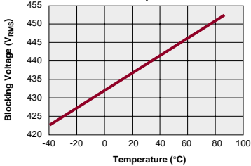
IAD170P Typical Blocking Voltage vs. Temperature
