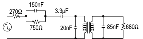
ESMIT-300 Optimal Circuit (Z=European Complex Impedance)
