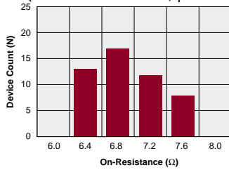
LAA127 Typical On-Resistance Distribution (N=50 Ambient Temperature = 25°C) (Load Current = 200mADC; I F = 5mADC)
