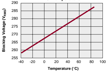
LAA127L Typical Blocking Voltage vs. Temperature
