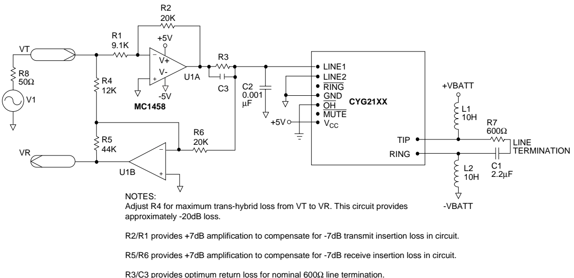
Figure 4. Hybrid Circuit
