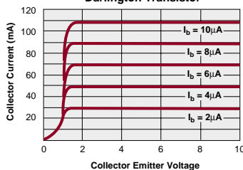
ITC117P/ITC135P/ITC137P Typical Transfer Characteristics of Darlington Transistor
