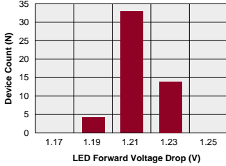
XBB170 Typical LED Forward Voltage Drop (N=50 Ambient Temperature = 25°C) I F = 5mADC
