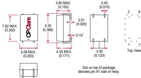
MRF4 Gull Wing (Lead Option -01)
