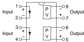
FDA215 Pinout
