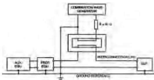
Figure 18. Test set-up for unshielded interconnection lines; line to line coupling according to 7.3; inductive coupling for high impedance circuits.
