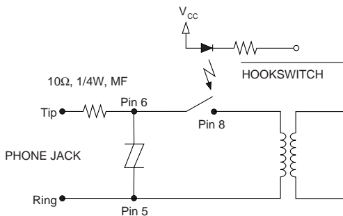
Figure 4. Typical Two Wire Application
