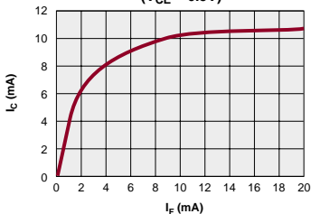
ITC117P/ITC135P/ITC137P Single Transistor Typical Collector Current vs. Forward Current ( V_{CE} = 0.5V )
