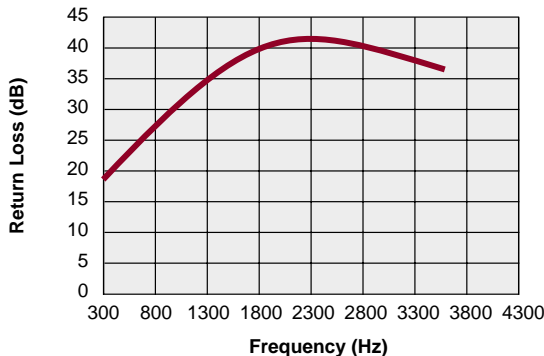
Figure 7. CYG21XX Series Return Loss
