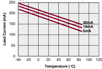
TS122 Typical Load Current vs. Temperature
