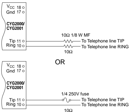
Figure 9. CYG20XX Fuse Requirements
