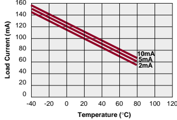
IAD170P Typical Load Current vs. Temperature
