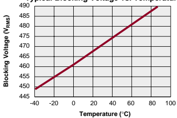
PAA110L Typical Blocking Voltage vs. Temperature
