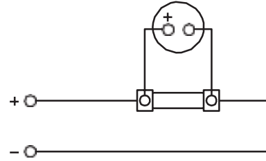
DC Amps - For use with external shunt
