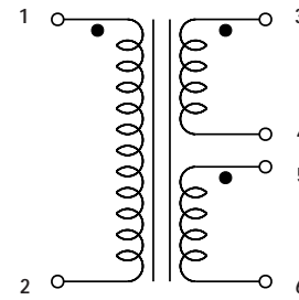
Schematic 2 (PCT-Series)
