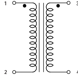
Schematic 4 (PCT-Series)
