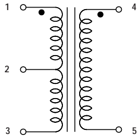
Schematic 3 (PCT-Series)
