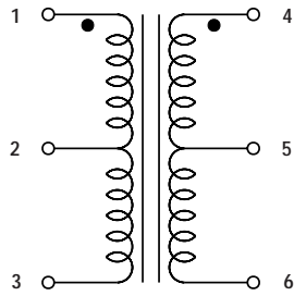
Schematic 1 (PCT-Series)
