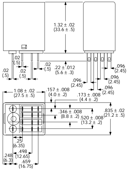
PCL 4c, 4a type (Plug-in Terminal)
