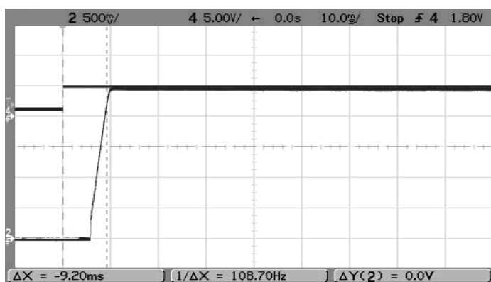
Step Load Transient Response (Vin=12V, Vout=2.5V, Cloud=0, Iout=3A to 6A)
