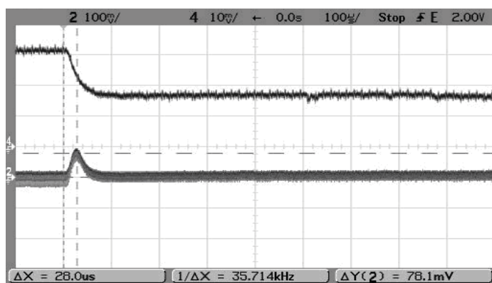
Step Load Transient Response (Vin=12V, Vout=2.5V, Cloud=0, Iout=6A to 3A)
