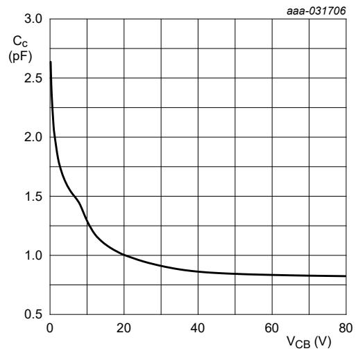
Fig. 14. NHUMH1: Collector capacitance as a function of collector-base voltage; typical values
